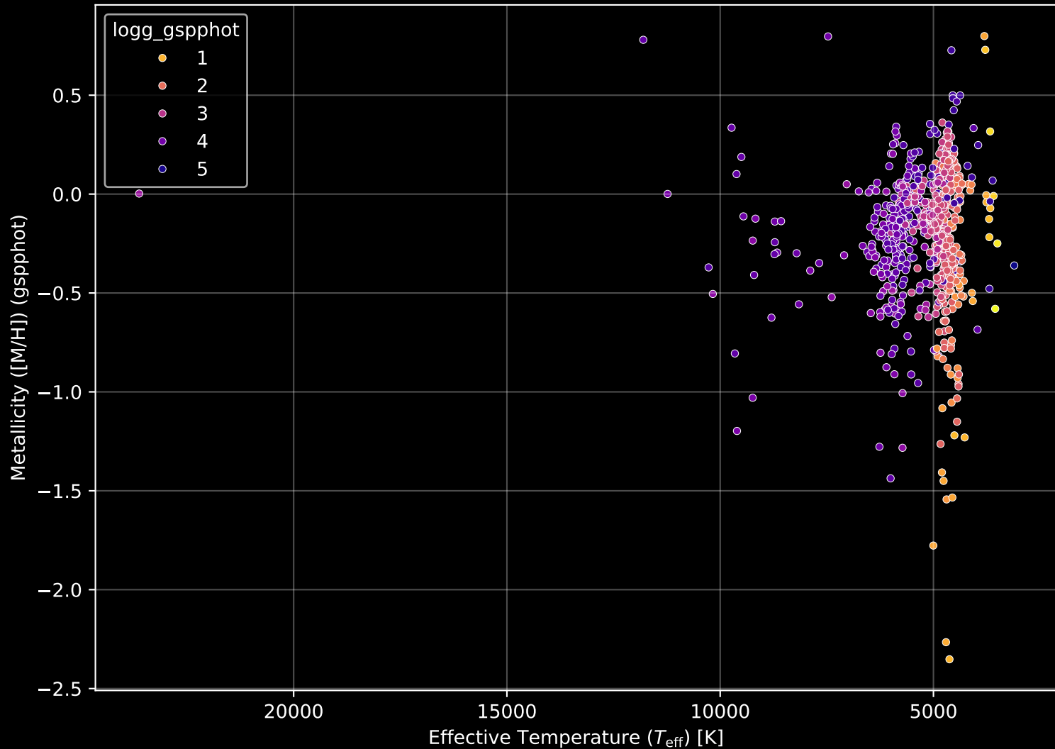
APOGEE DR17 Field: [K09_081+11] Stellar Population Parameters (n= 829)
