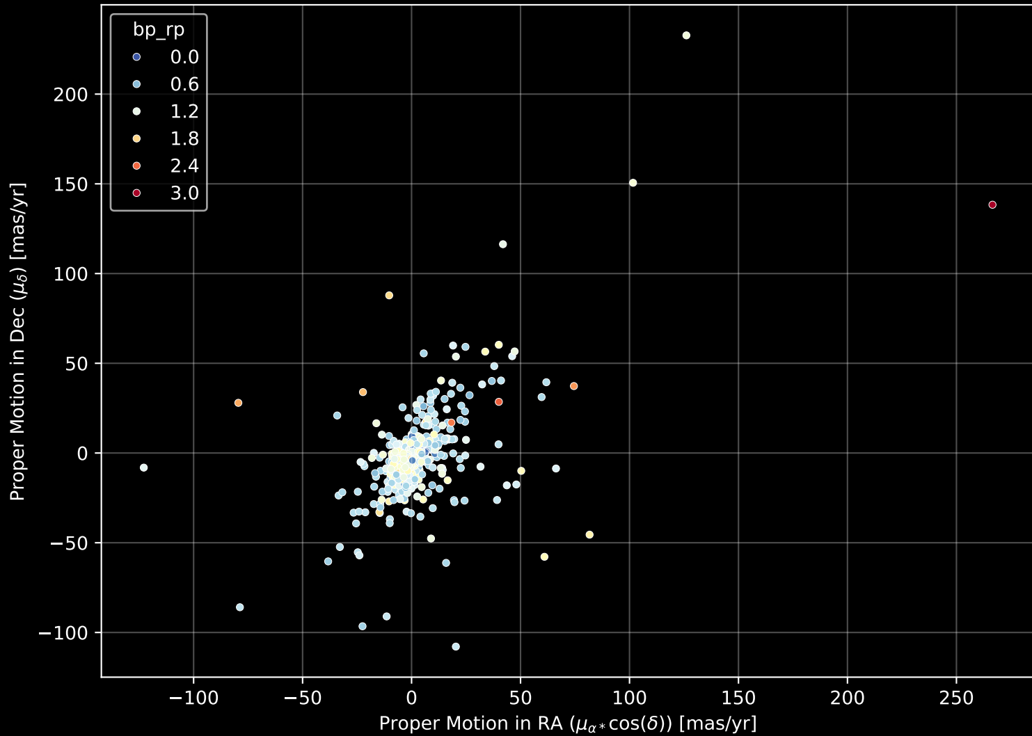
APOGEE DR17 Field: [K09_081+11] Proper Motion Diagram (n= 829)
