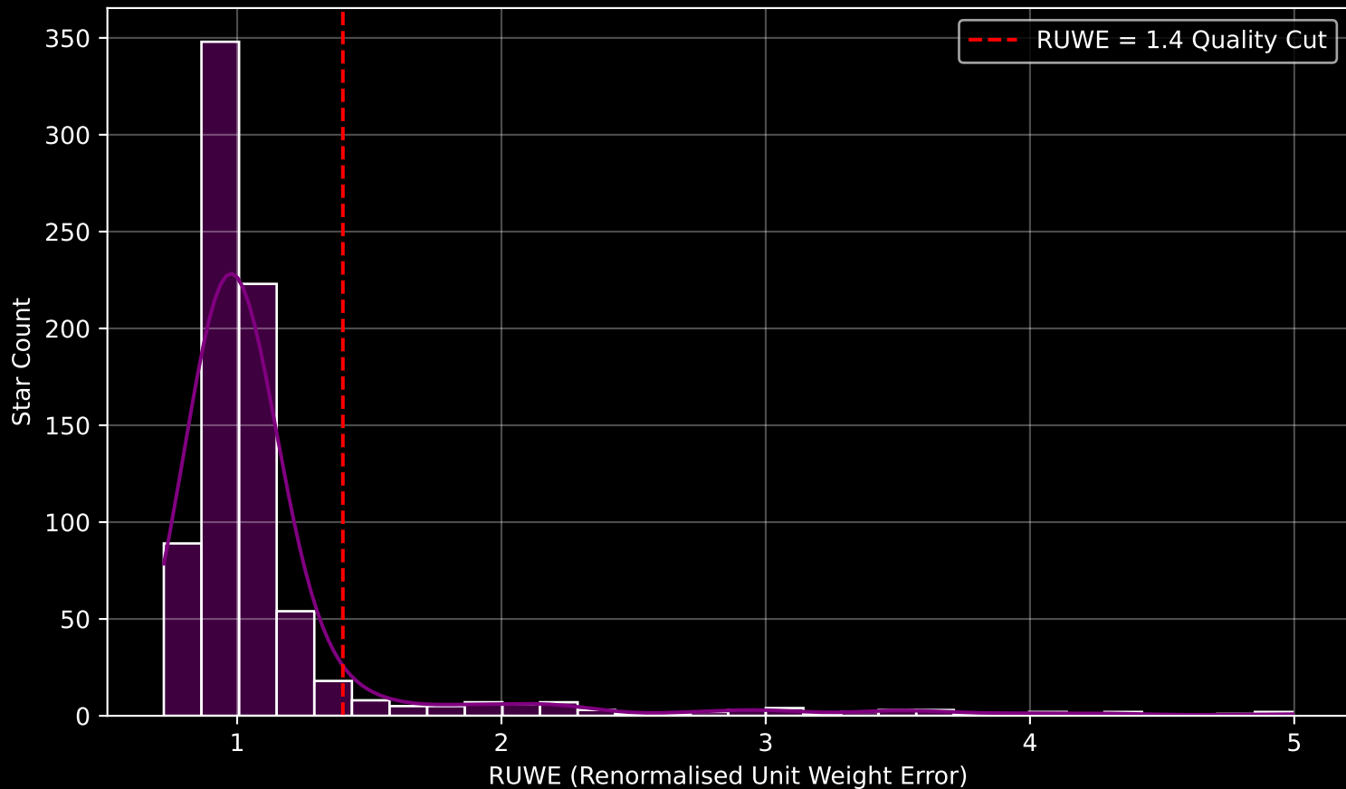
GAPOGEE DR17 Field [K09_081+11] RUWE Distribution (n= 803)
