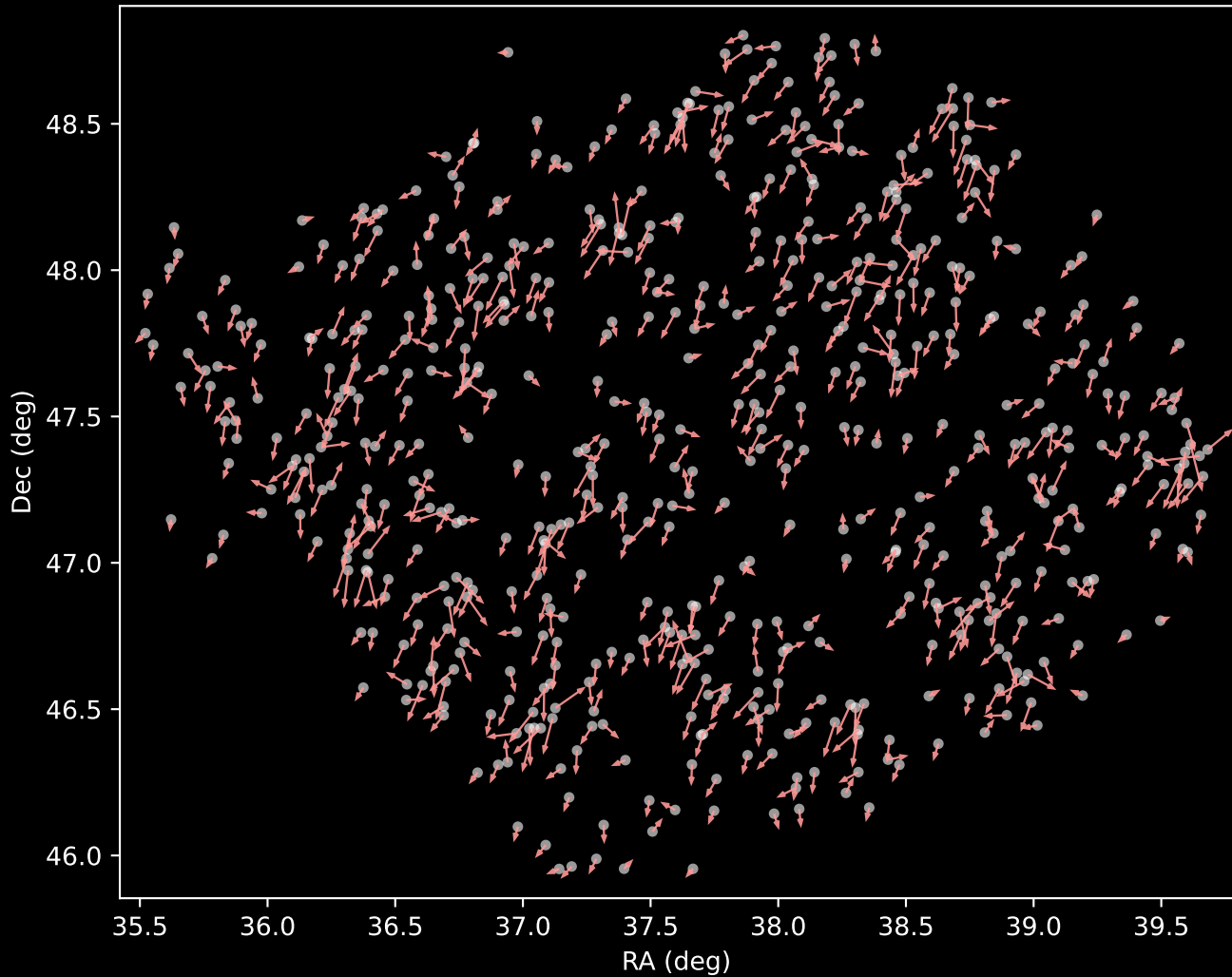
APOGEE DR17 Cluster 7 Proper Motion Vectors (n=595)
