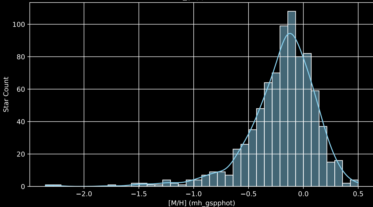
APOGEE DR17 Field: [K09_081+11 [M/H] (mh_gspphot) (n= 824)
