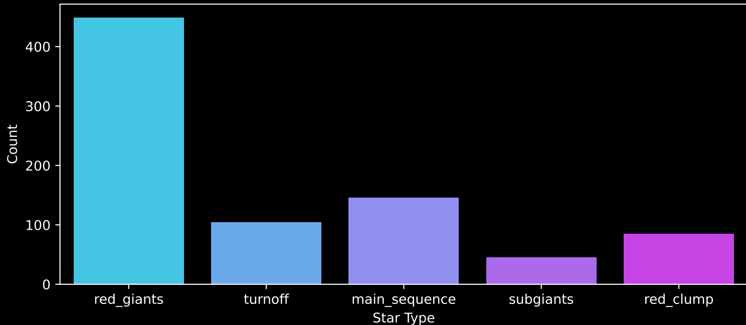
APOGEE DR17 Field: [K09_081+11] Count plot of Star Type
