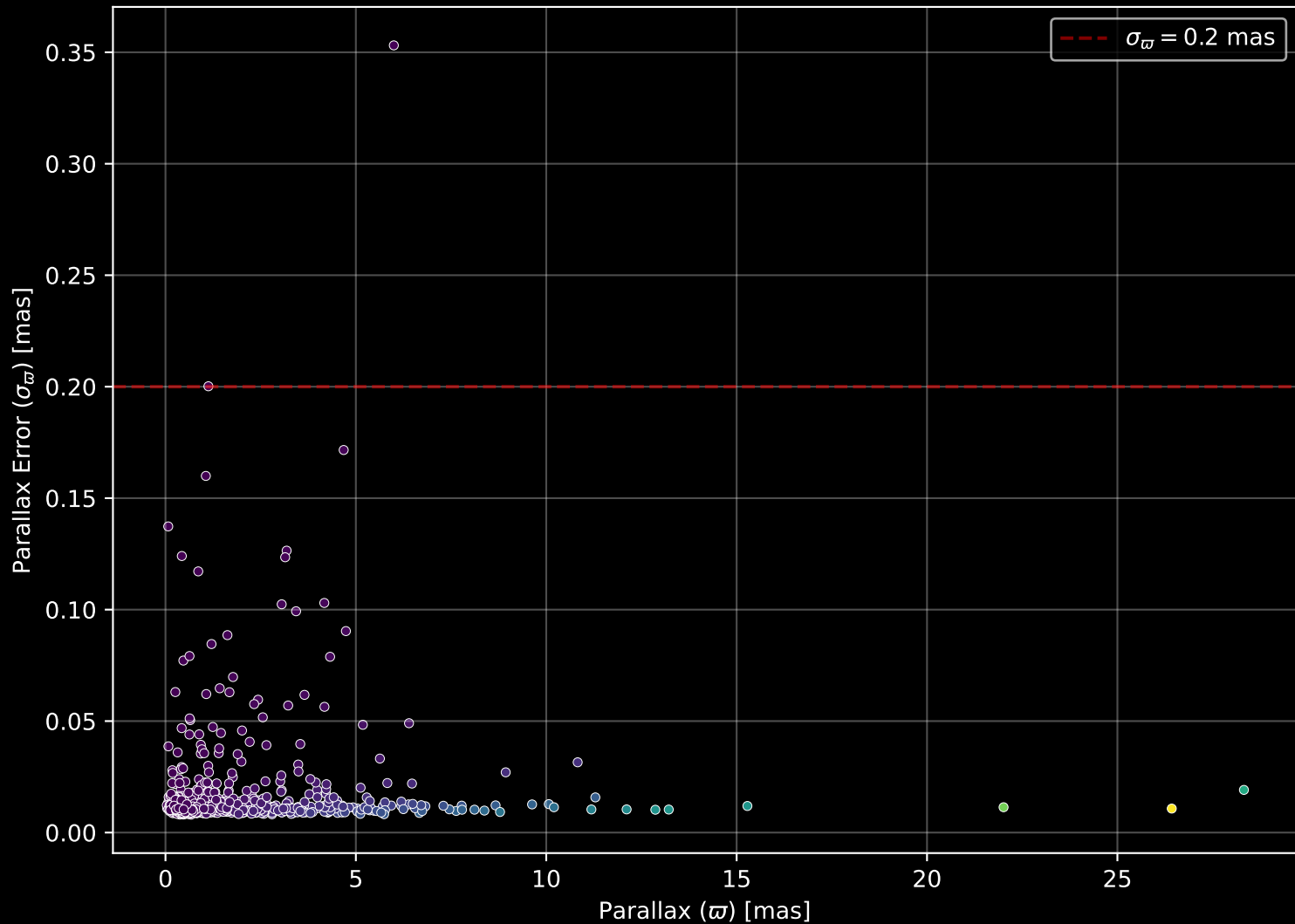
APOGEE DR17 Field: [K09_081+11] Parallax Quality (n= 829)
